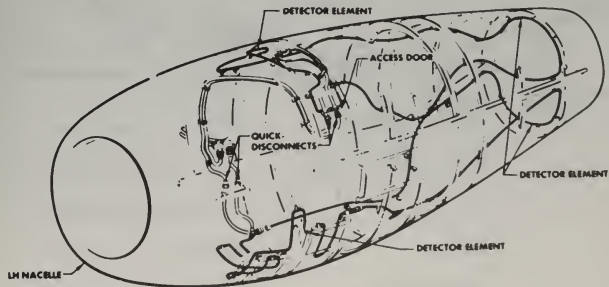
FIGURE 9-23. Fire detection system.
